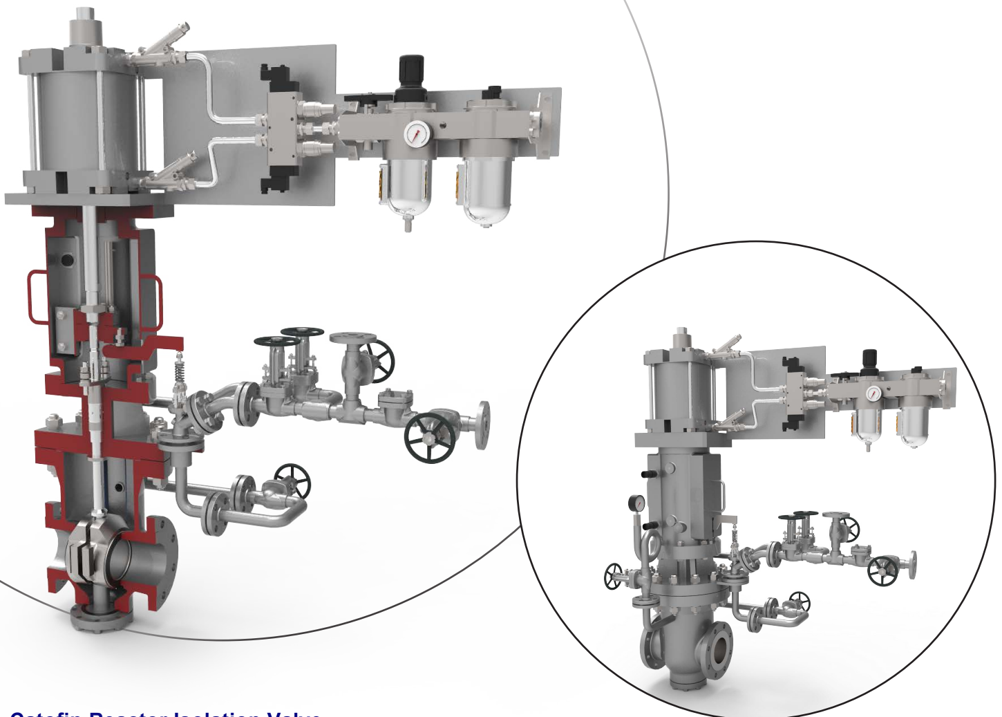
Catofin Reactor Isolation Valve
